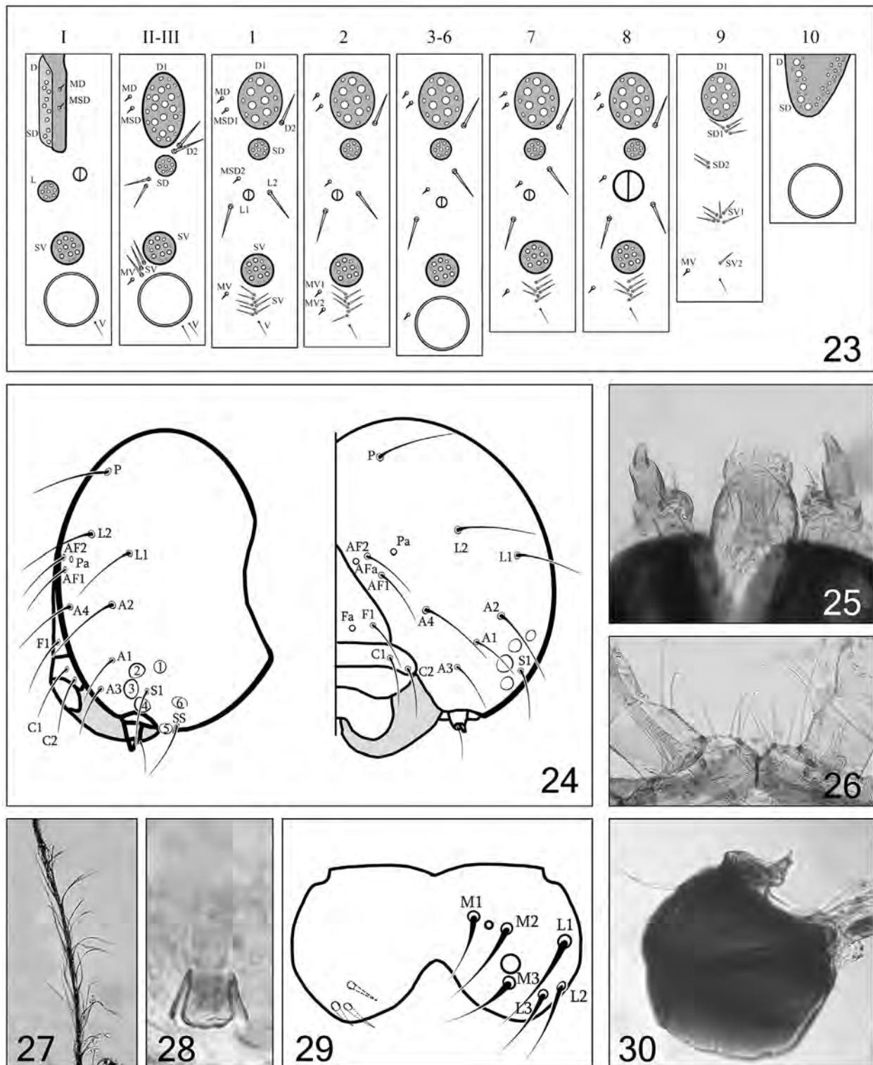
Figs 23–30. Structural details of Striphnopteryx edulis , L1. 23. setal map of body segments; 24. setal arrangement on head; 25. labio-maxillary complex; 26. fore legs showing fused coxae; 27. plumose (?subprimary) seta; 28. base of seta; 29. setal arrangement on labrum; 30. mandible.
