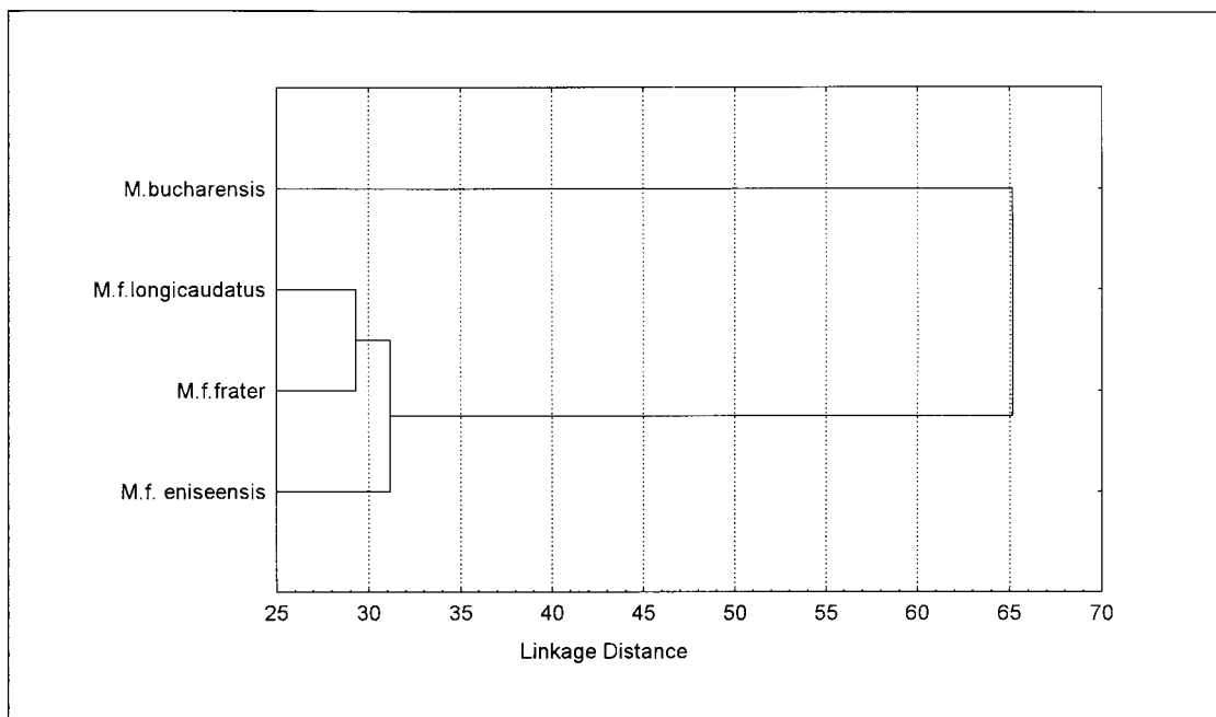
Fig. 6. Single linkage tree showing dissimilarities from matrix.
