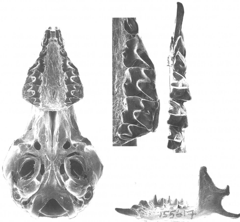
Fig. 1: Myosorex kihalei n. sp., paratype FMNH 155617; cranium in ventral view and left ramus of mandible in labial view, details of the dentition enlarged. SEM-photographs of uncoated skull.
