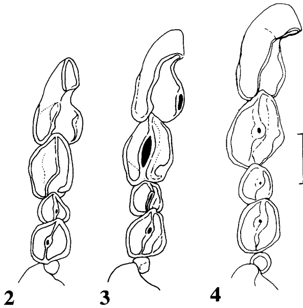
Figs. 2–4: Front dentition of right upper tooththrow in occlusal view. 2, Myosorex kahaulei n. sp. (RUCA 10984), 3, M. geata (RUCA 2305), 4, M. zinki (holotype SMNS 4505 reversed). Scale is 1 mm. Note the position of the fourth unicuspid tooth
