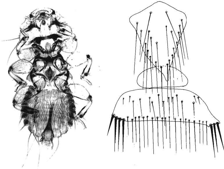
Abb. 13: Myrsidea sp. ♂
